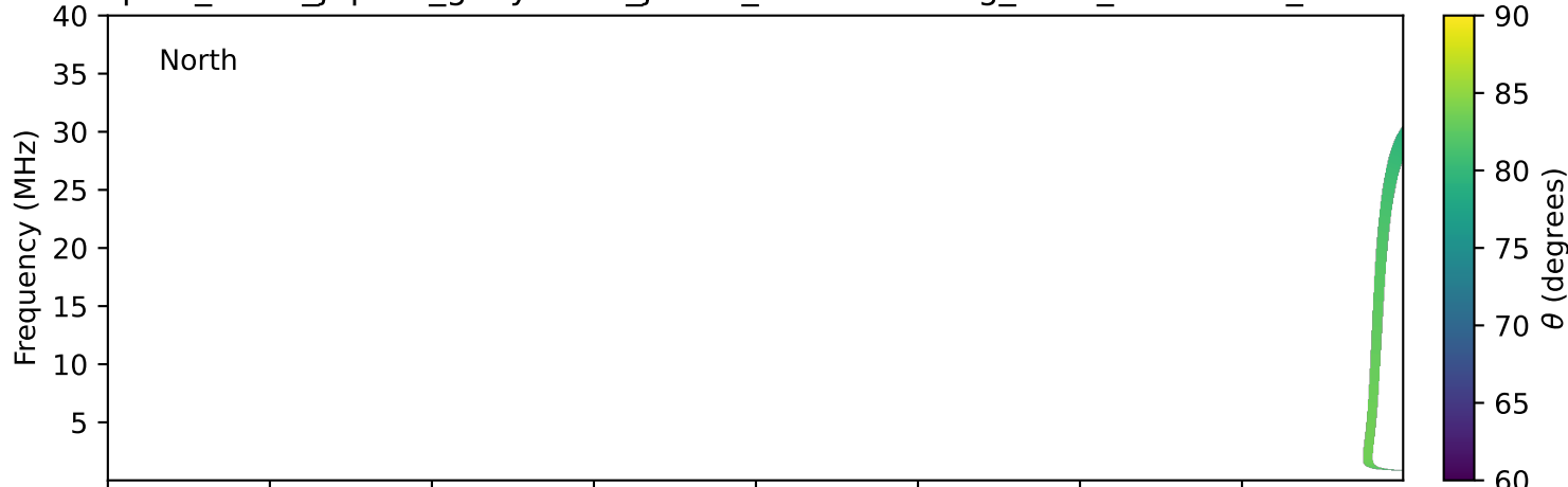
expres_earth_jupiter_ganymede_jrm09_lossc-wid1deg_3kev_20231101_v11.cdf
