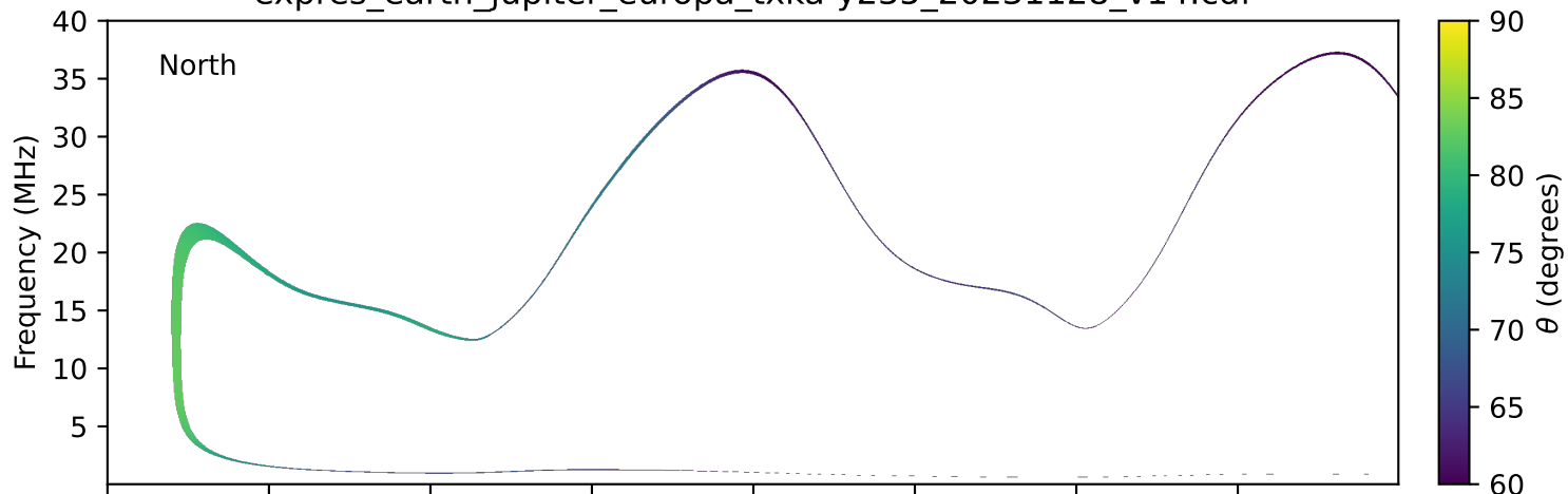
expres_earth_jupiter_europa_txka-y235_20231128_v14.cdf
