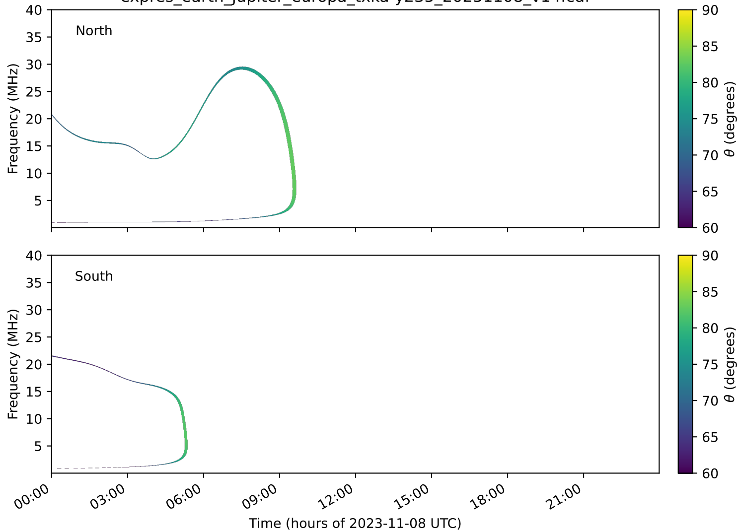
expres_earth_jupiter_europa_txka-y235_20231108_v14.cdf
