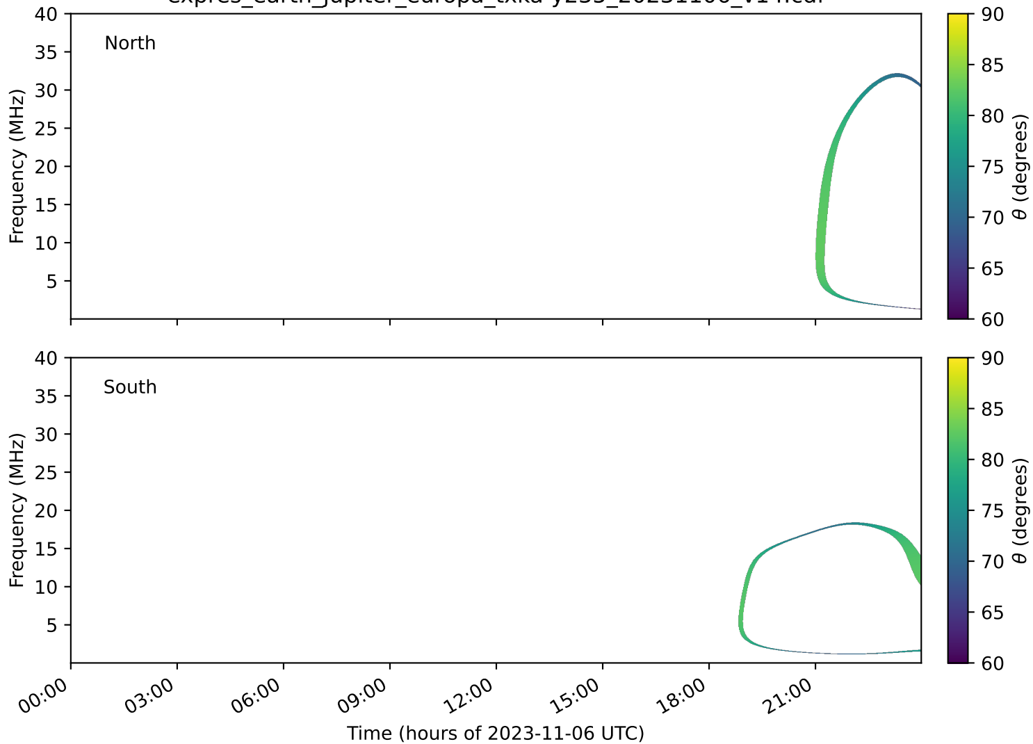
expres_earth_jupiter_europa_txka-y235_20231106_v14.cdf
