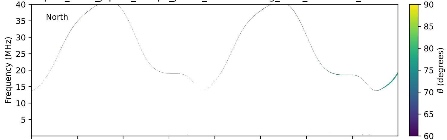
expres_earth_jupiter_europa_jrm33_lossc-wid1deg_3kev_20231125_v11.cdf
