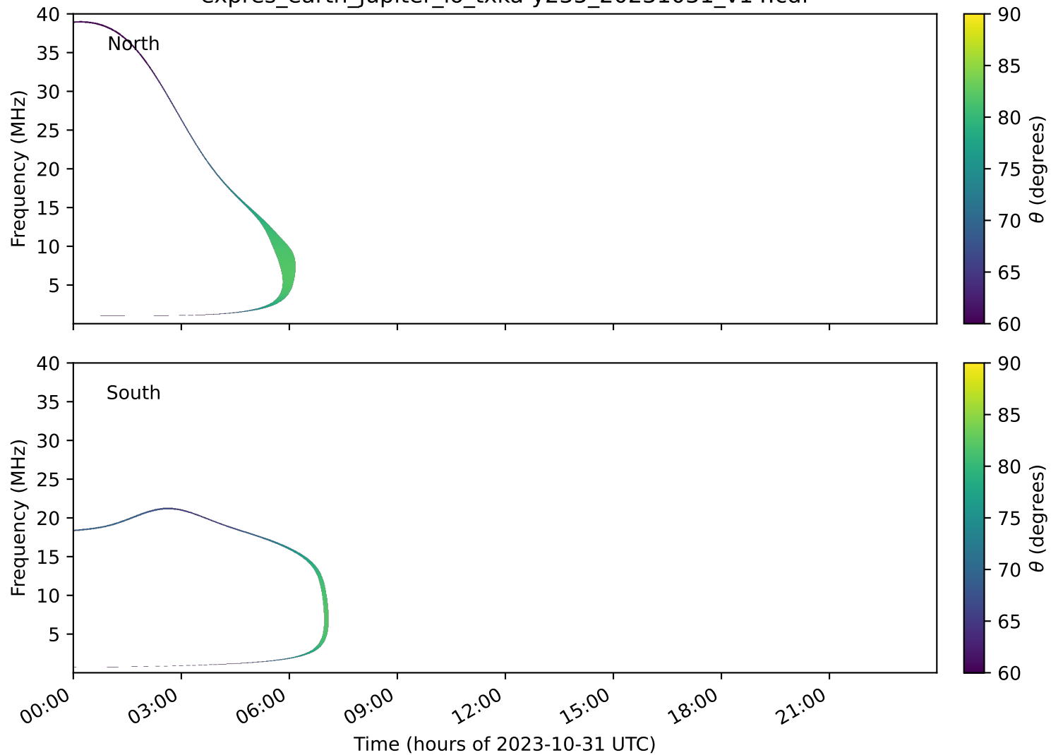
expres_earth_jupiter_io_txka-y235_20231031_v14.cdf
