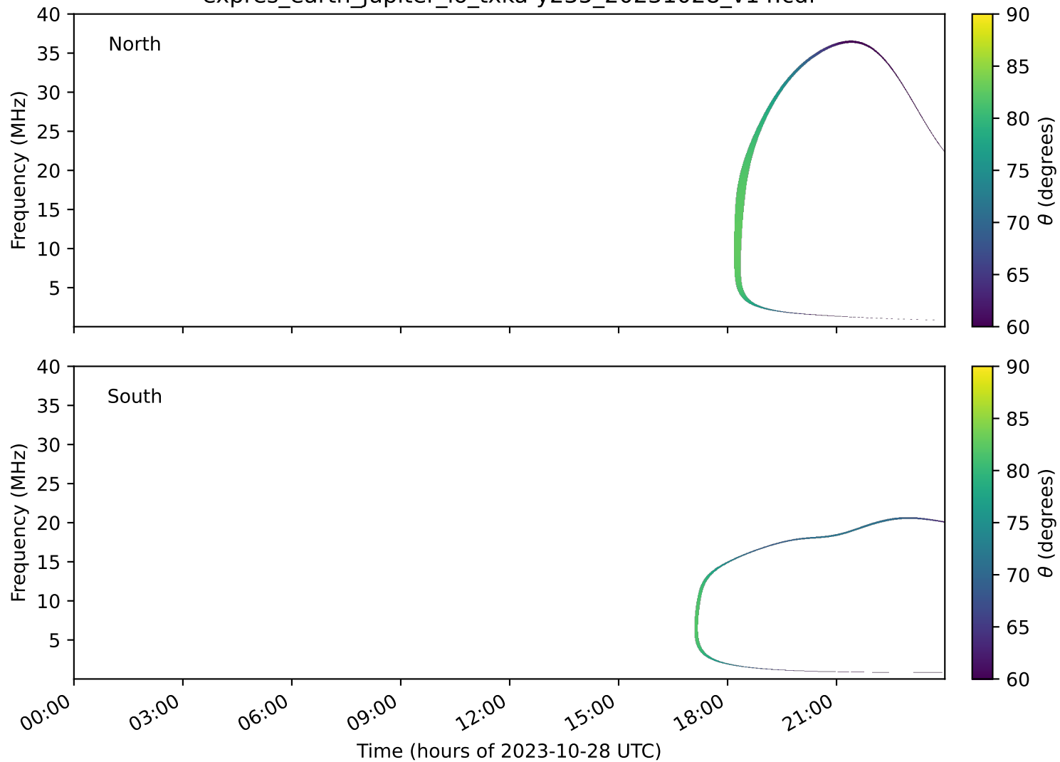
expres_earth_jupiter_io_txka-y235_20231028_v14.cdf
