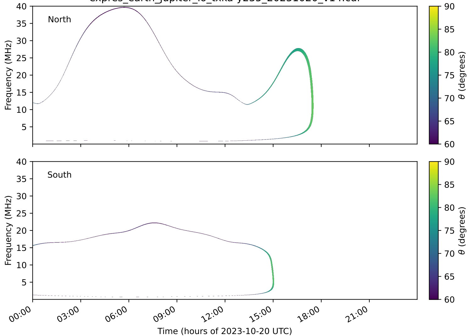
expres_earth_jupiter_io_txka-y235_20231020_v14.cdf
