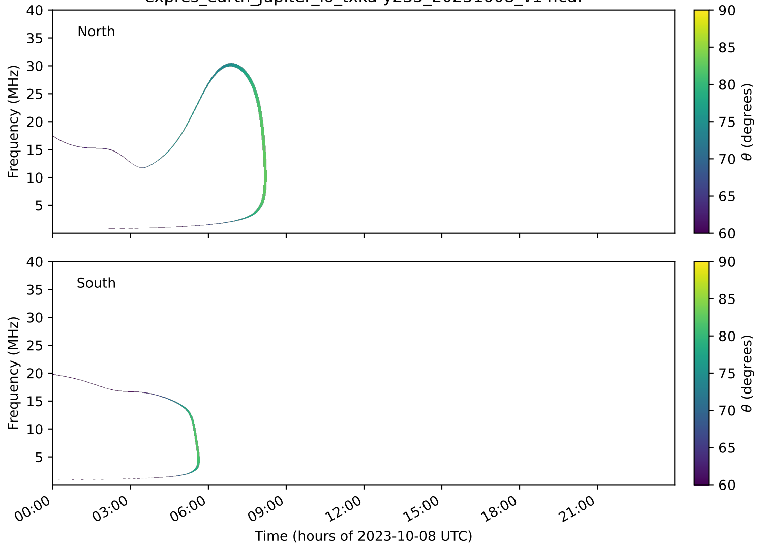
expres_earth_jupiter_io_txka-y235_20231008_v14.cdf
