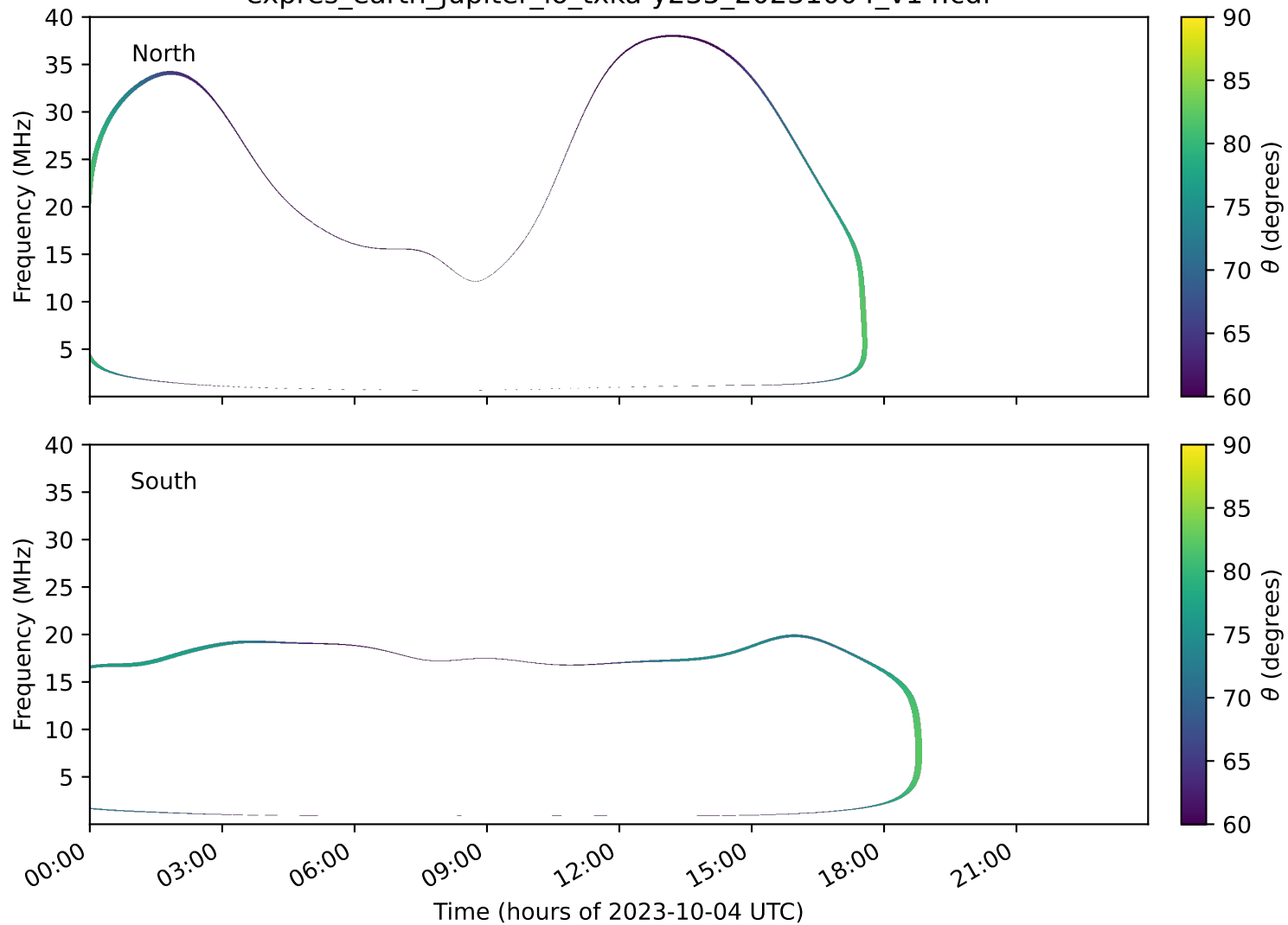
expres_earth_jupiter_io_txka-y235_20231004_v14.cdf
