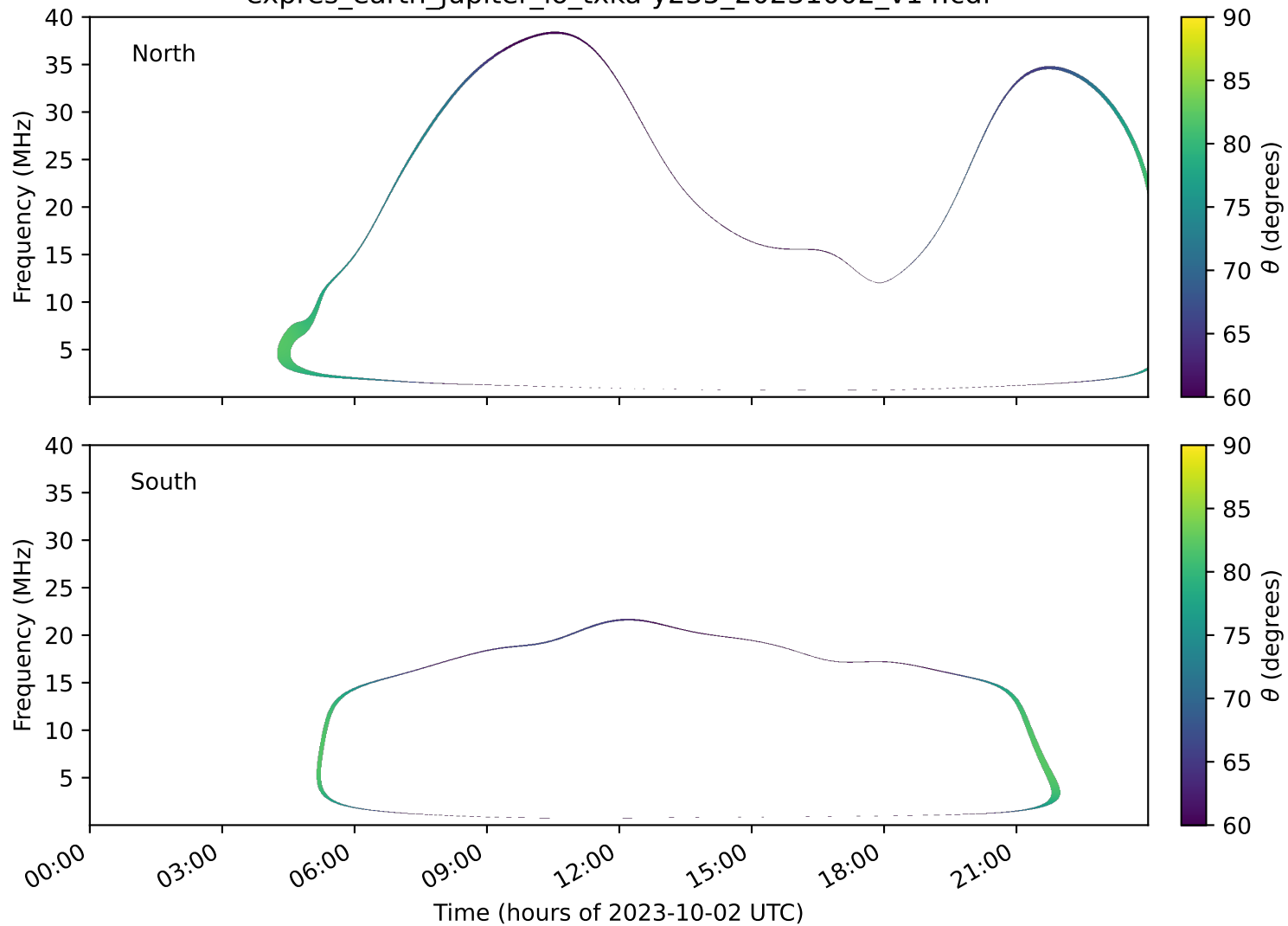
expres_earth_jupiter_io_txka-y235_20231002_v14.cdf
