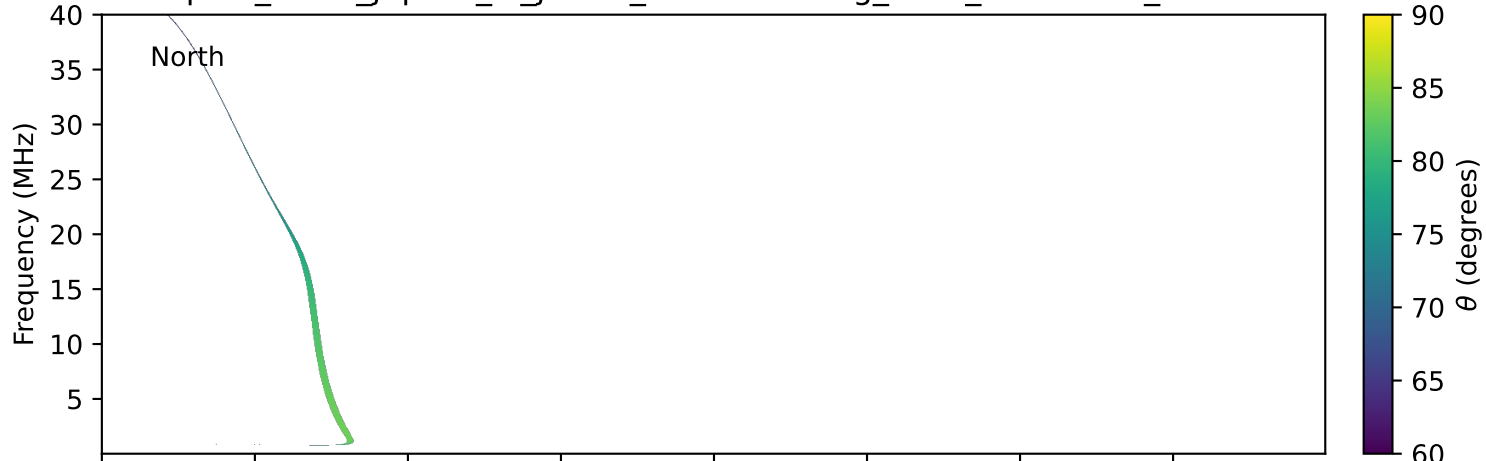
expres_earth_jupiter_io_jrm33_lossc-wid1deg_3kev_20231024_v11.cdf
