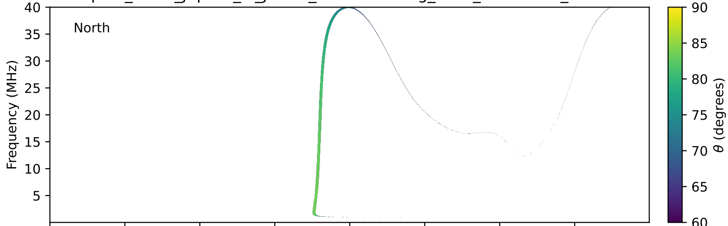
expres_earth_jupiter_io_jrm33_lossc-wid1deg_3kev_20231023_v11.cdf
