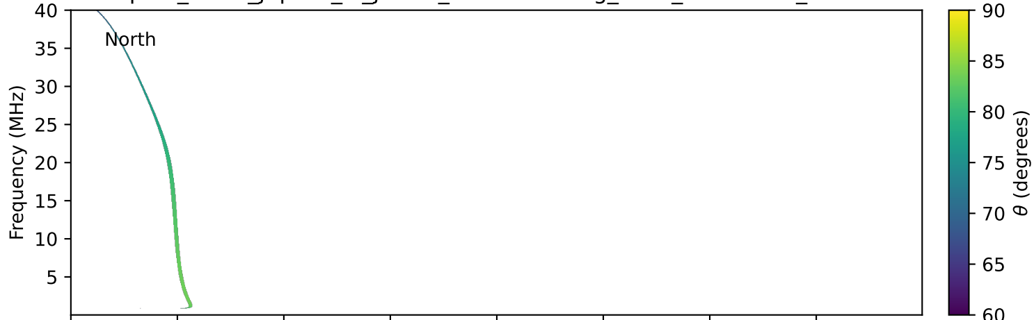
expres_earth_jupiter_io_jrm33_lossc-wid1deg_3kev_20231017_v11.cdf
