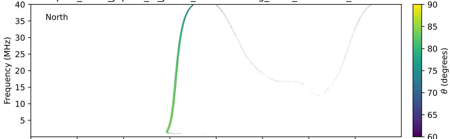
expres_earth_jupiter_io_jrm33_lossc-wid1deg_3kev_20231016_v11.cdf
