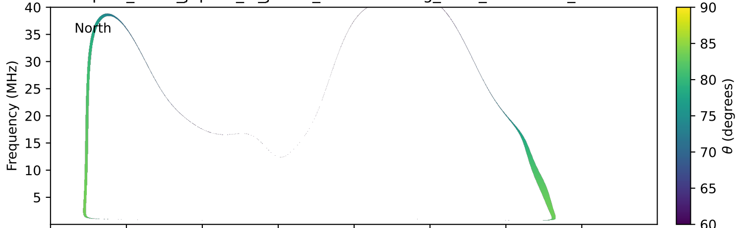
expres_earth_jupiter_io_jrm33_lossc-wid1deg_3kev_20231011_v11.cdf
