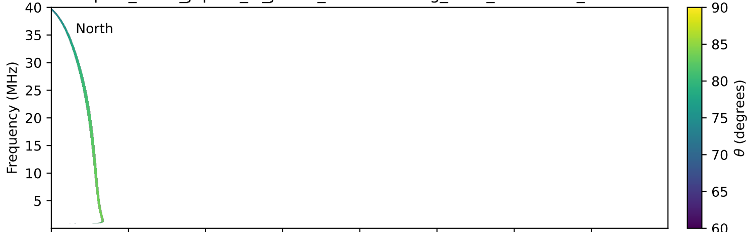
expres_earth_jupiter_io_jrm33_lossc-wid1deg_3kev_20231010_v11.cdf
