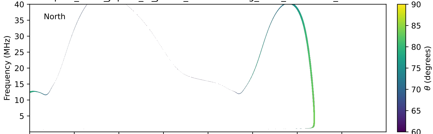
expres_earth_jupiter_io_jrm09_lossc-wid1deg_3kev_20231027_v11.cdf
