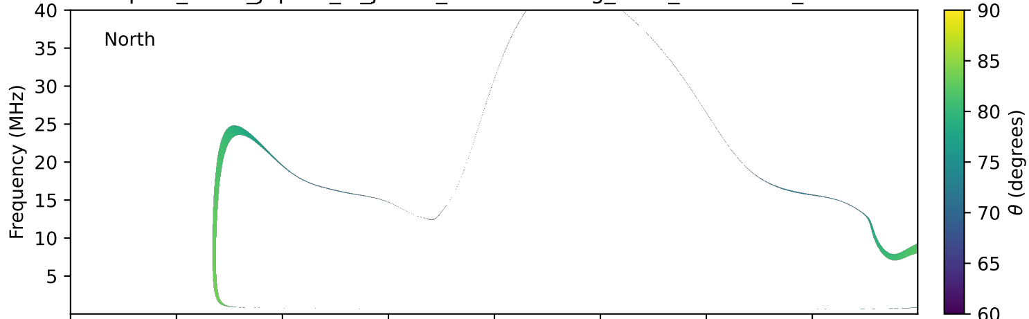
expres_earth_jupiter_io_jrm09_lossc-wid1deg_3kev_20231025_v11.cdf
