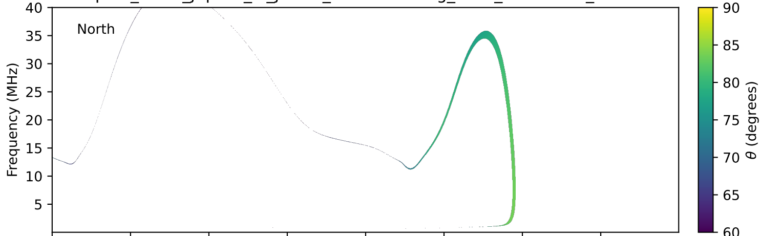
expres_earth_jupiter_io_jrm09_lossc-wid1deg_3kev_20231020_v11.cdf
