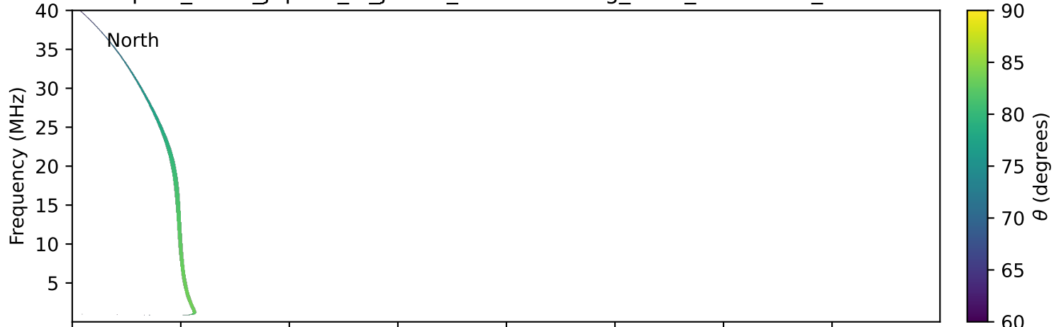
expres_earth_jupiter_io_jrm09_lossc-wid1deg_3kev_20231017_v11.cdf
