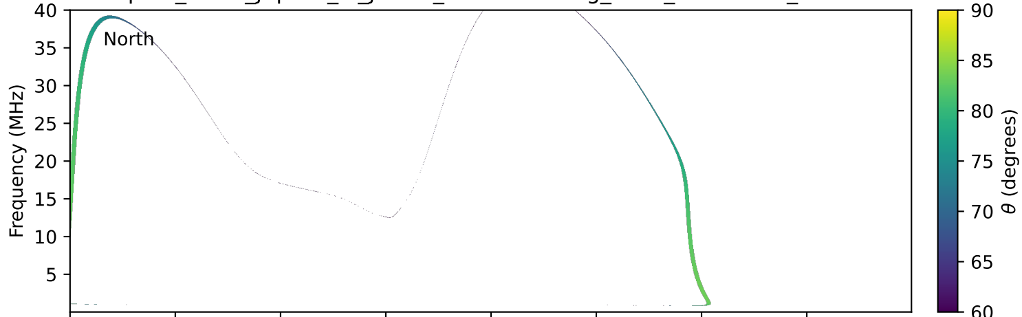
expres_earth_jupiter_io_jrm09_lossc-wid1deg_3kev_20231004_v11.cdf
