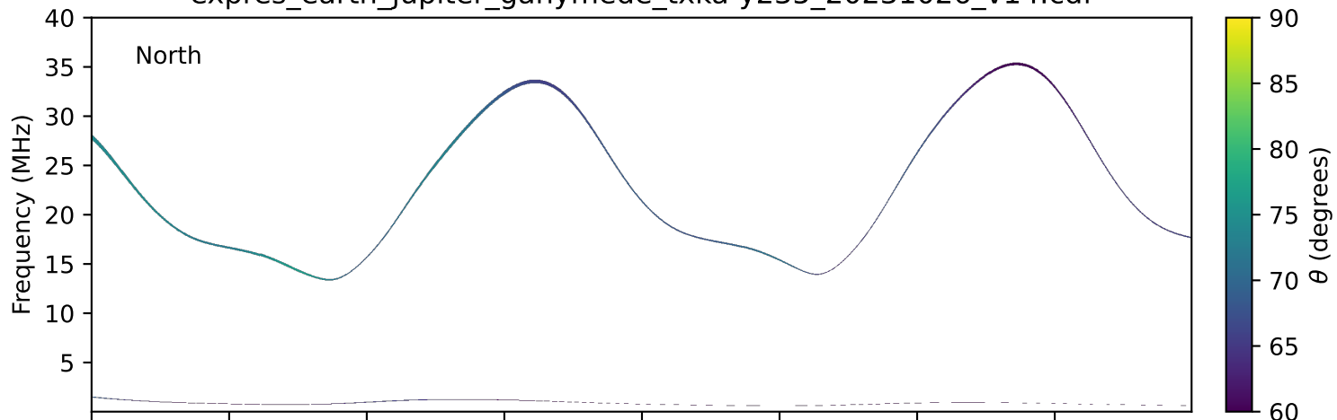
expres_earth_jupiter_ganymede_txka-y235_20231026_v14.cdf
