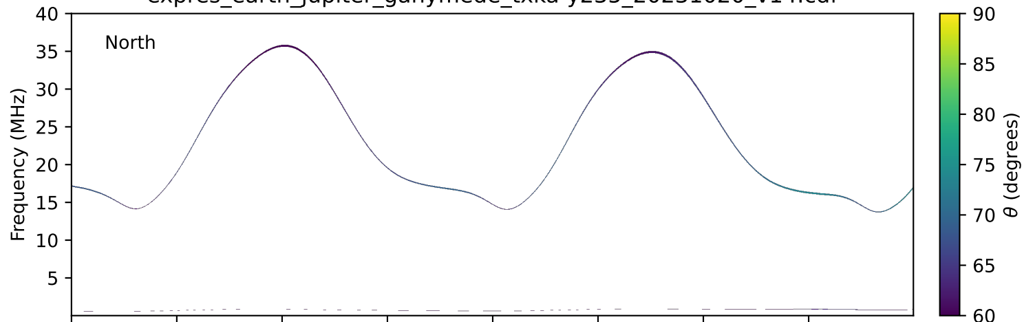
expres_earth_jupiter_ganymede_txka-y235_20231020_v14.cdf
