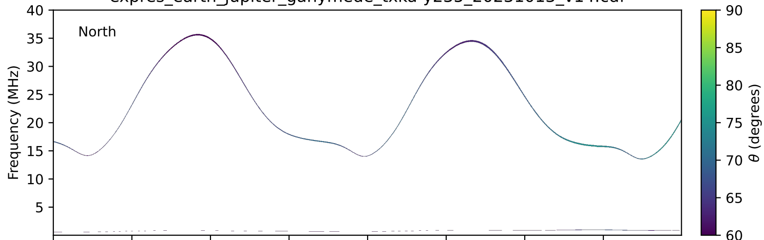
expres_earth_jupiter_ganymede_txka-y235_20231013_v14.cdf
