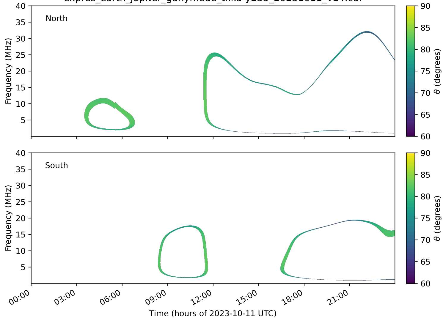
expres_earth_jupiter_ganymede_txka-y235_20231011_v14.cdf
