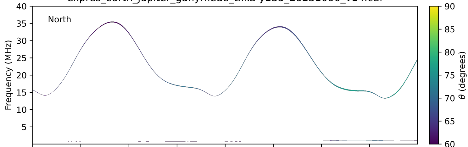
expres_earth_jupiter_ganymede_txka-y235_20231006_v14.cdf
