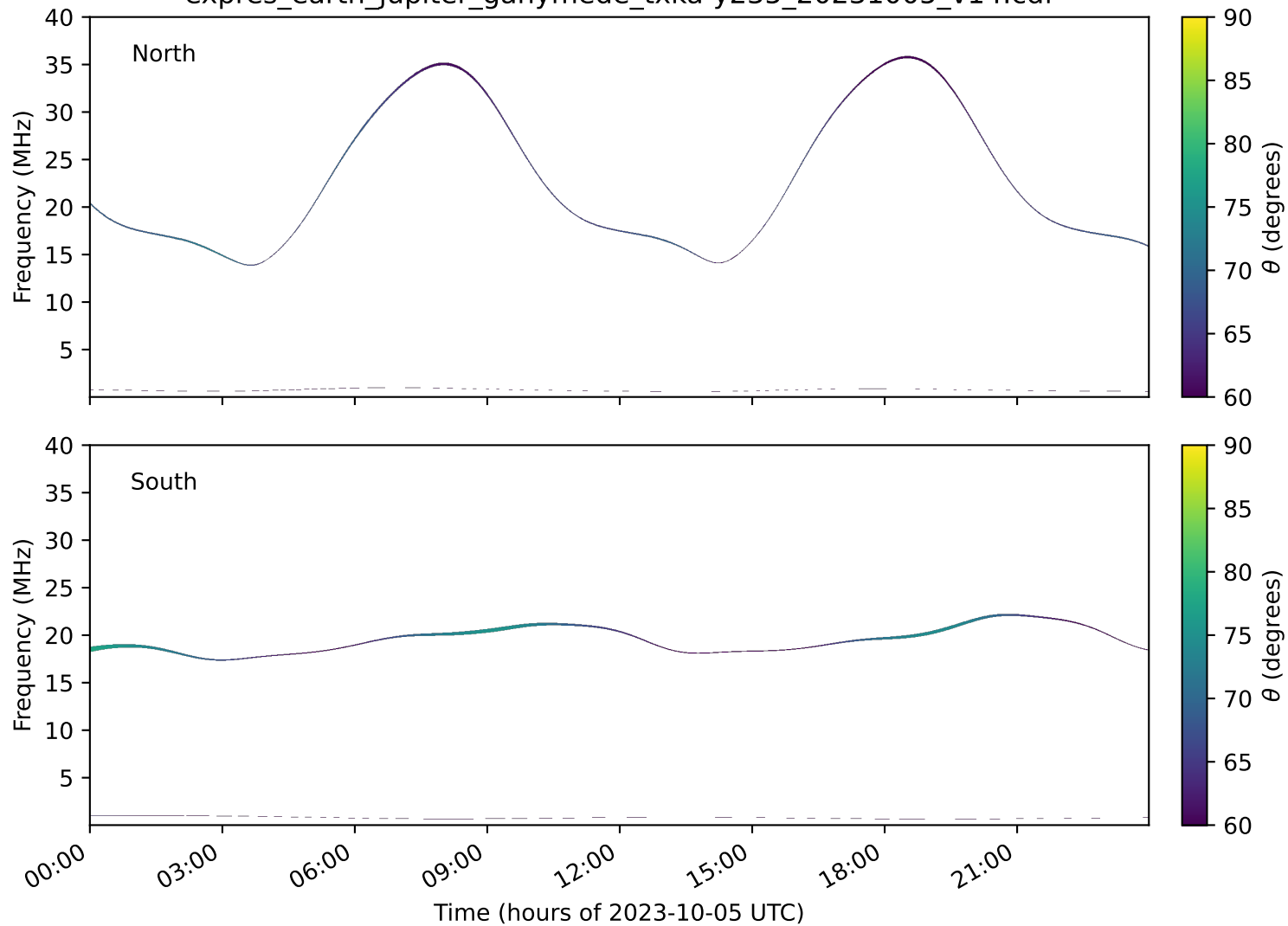
expres_earth_jupiter_ganymede_txka-y235_20231005_v14.cdf
