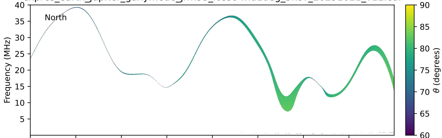
expres_earth_jupiter_ganymede_jrm33_lossc-wid1deg_3kev_20231021_v11.cdf
