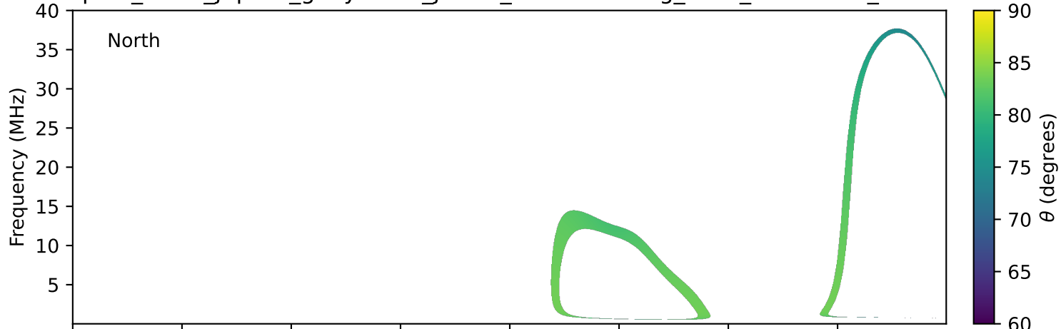
expres_earth_jupiter_ganymede_jrm33_lossc-wid1deg_3kev_20231018_v11.cdf
