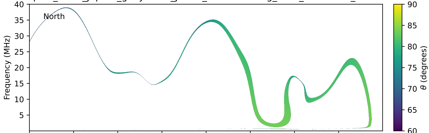
expres_earth_jupiter_ganymede_jrm33_lossc-wid1deg_3kev_20231014_v11.cdf
