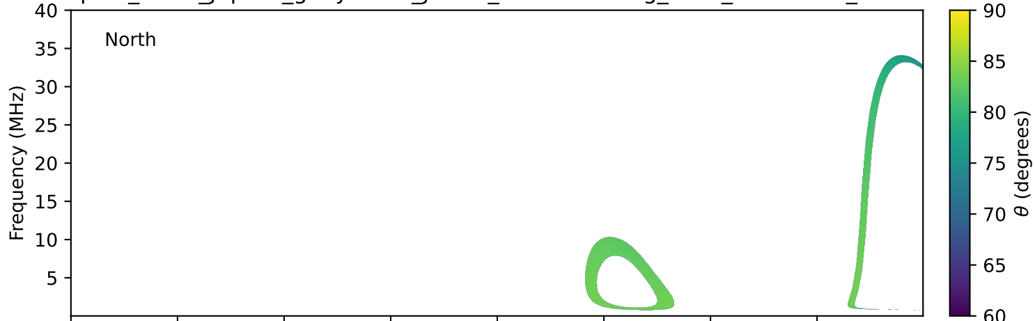
expres_earth_jupiter_ganymede_jrm09_lossc-wid1deg_3kev_20231025_v11.cdf
