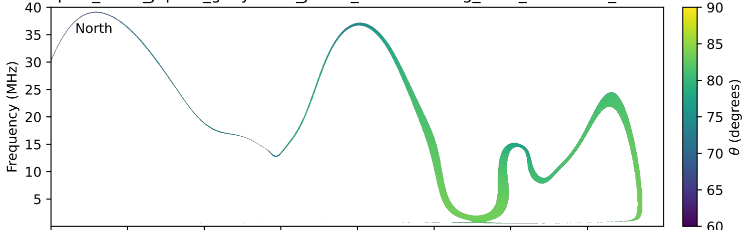
expres_earth_jupiter_ganymede_jrm09_lossc-wid1deg_3kev_20231014_v11.cdf
