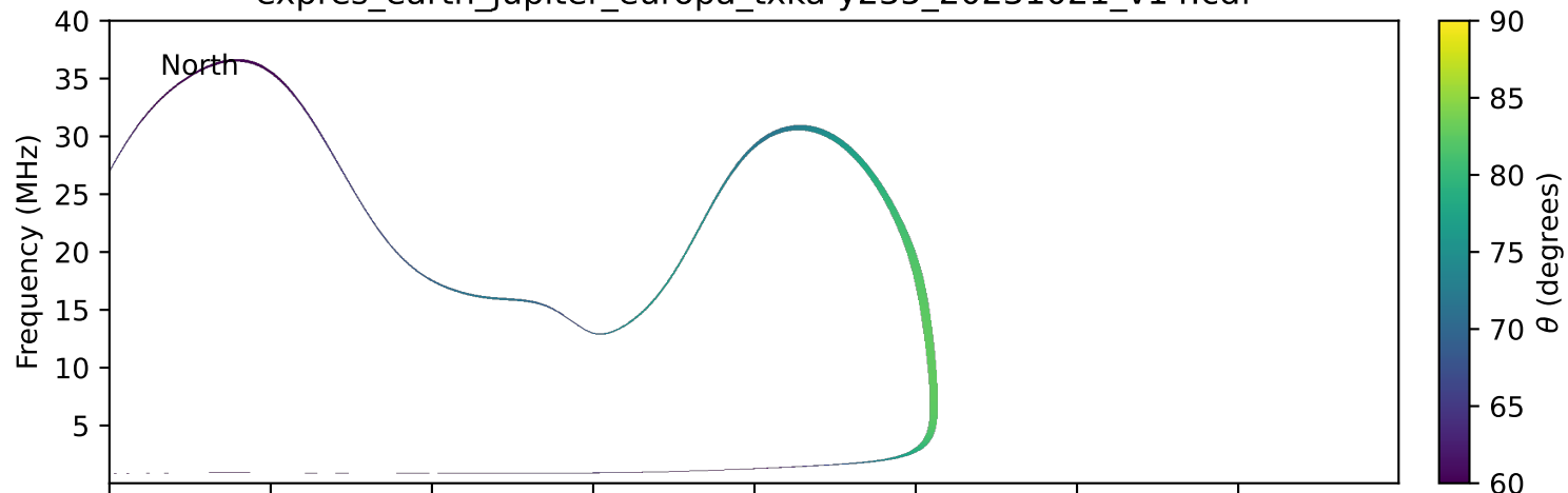
expres_earth_jupiter_europa_txka-y235_20231021_v14.cdf
