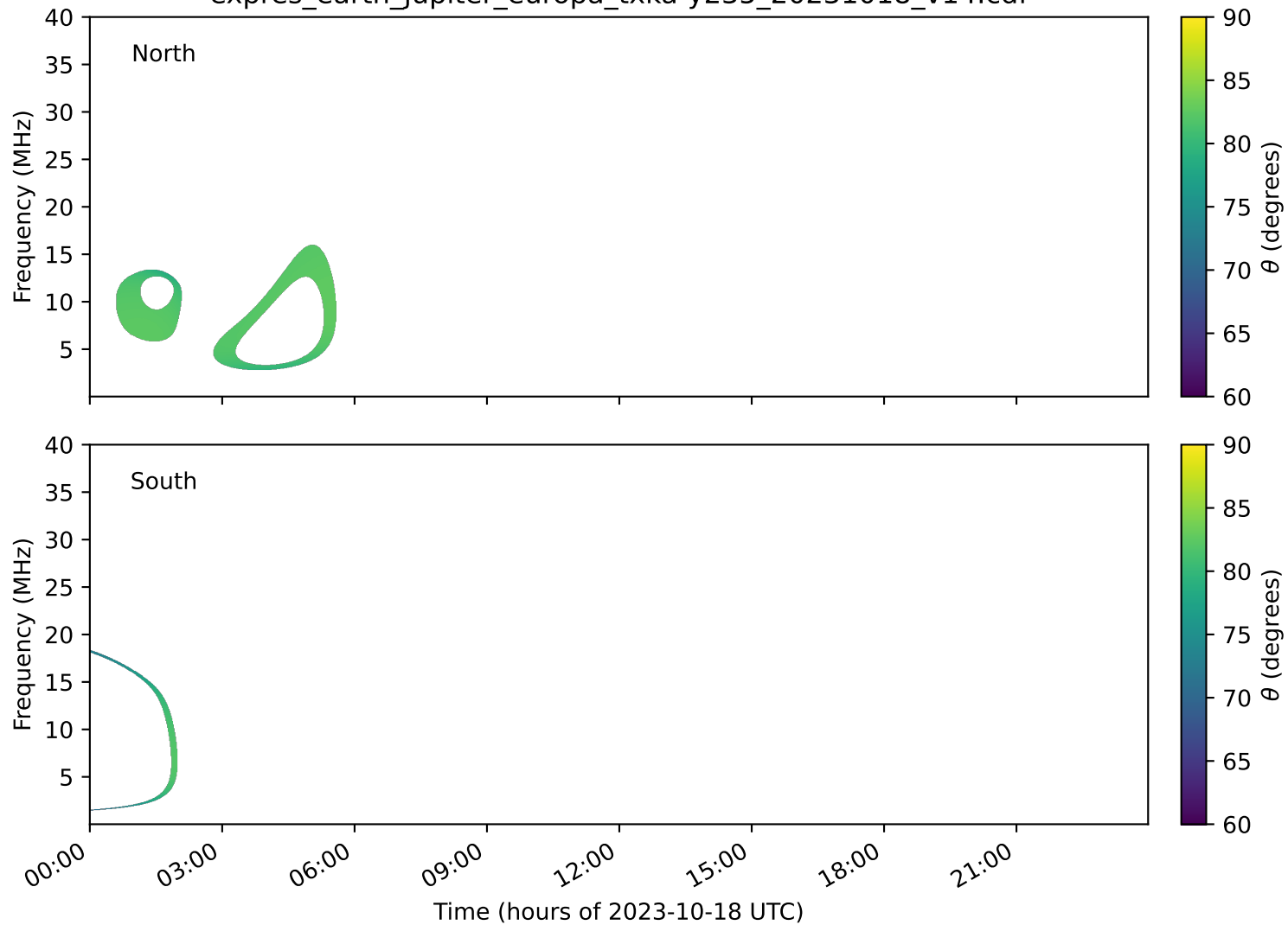
expres_earth_jupiter_europa_txka-y235_20231018_v14.cdf
