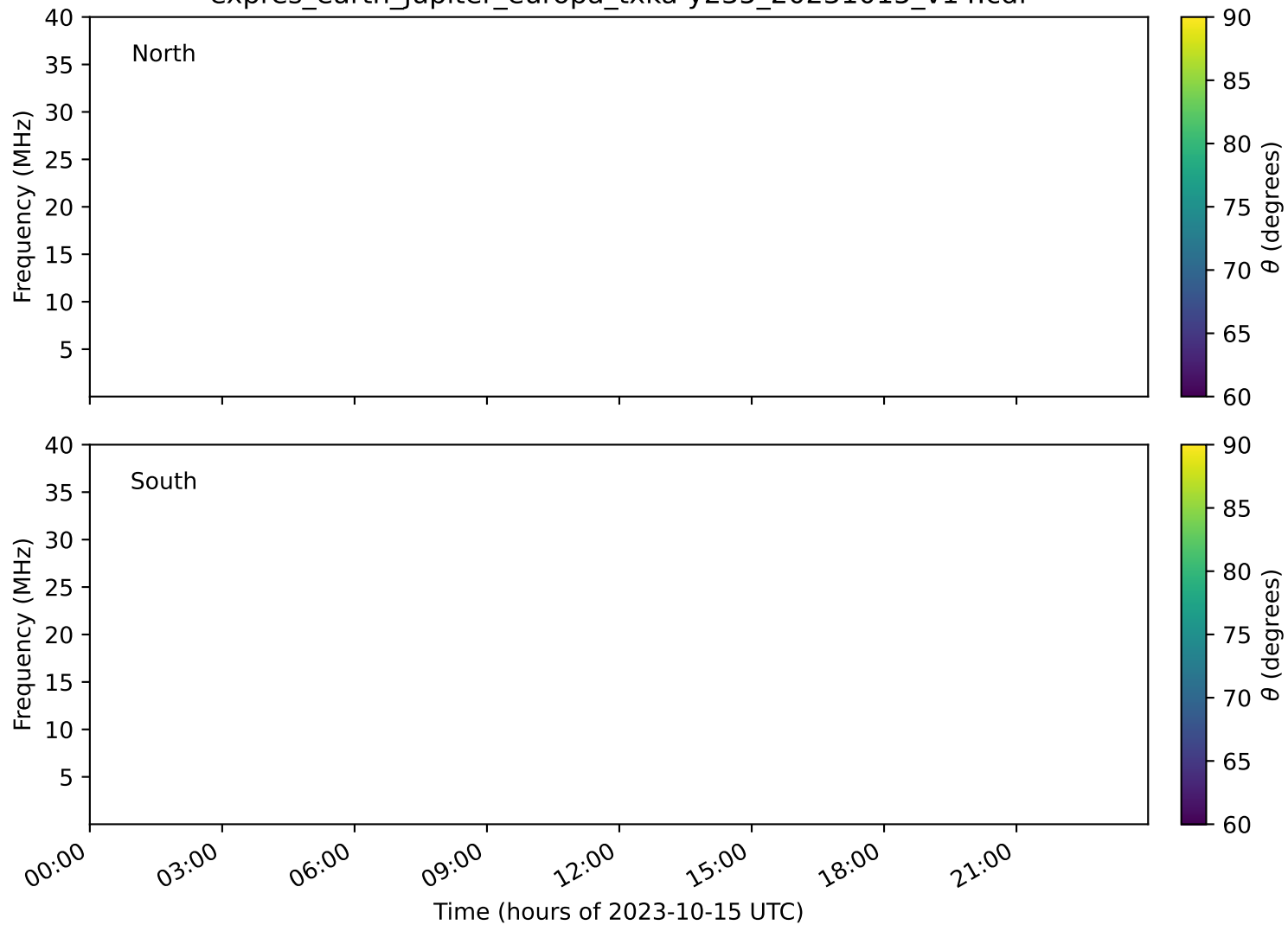
expres_earth_jupiter_europa_txka-y235_20231015_v14.cdf
