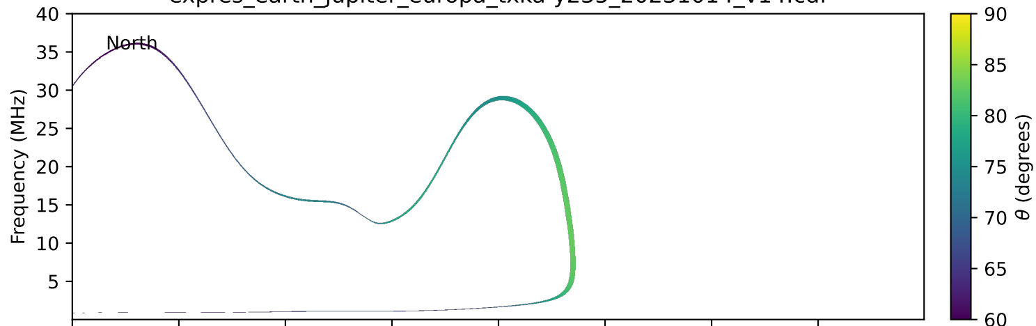
expres_earth_jupiter_europa_txka-y235_20231014_v14.cdf
