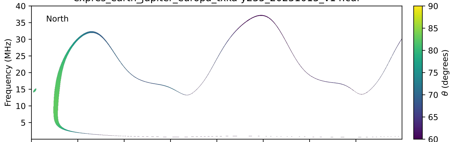
expres_earth_jupiter_europa_txka-y235_20231013_v14.cdf
