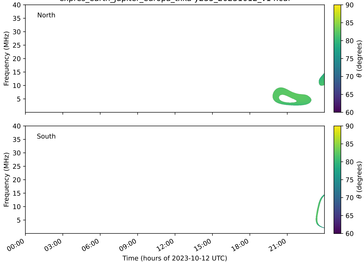
expres_earth_jupiter_europa_txka-y235_20231012_v14.cdf
