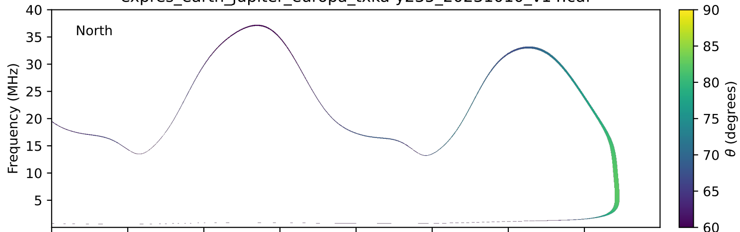
expres_earth_jupiter_europa_txka-y235_20231010_v14.cdf
