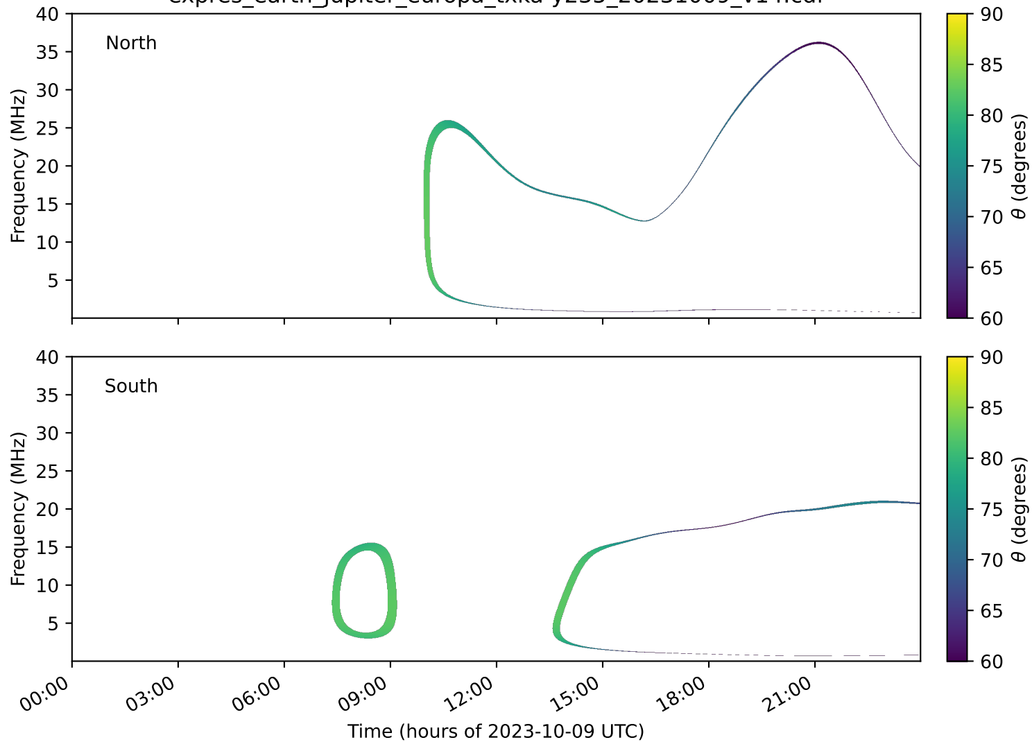
expres_earth_jupiter_europa_txka-y235_20231009_v14.cdf
