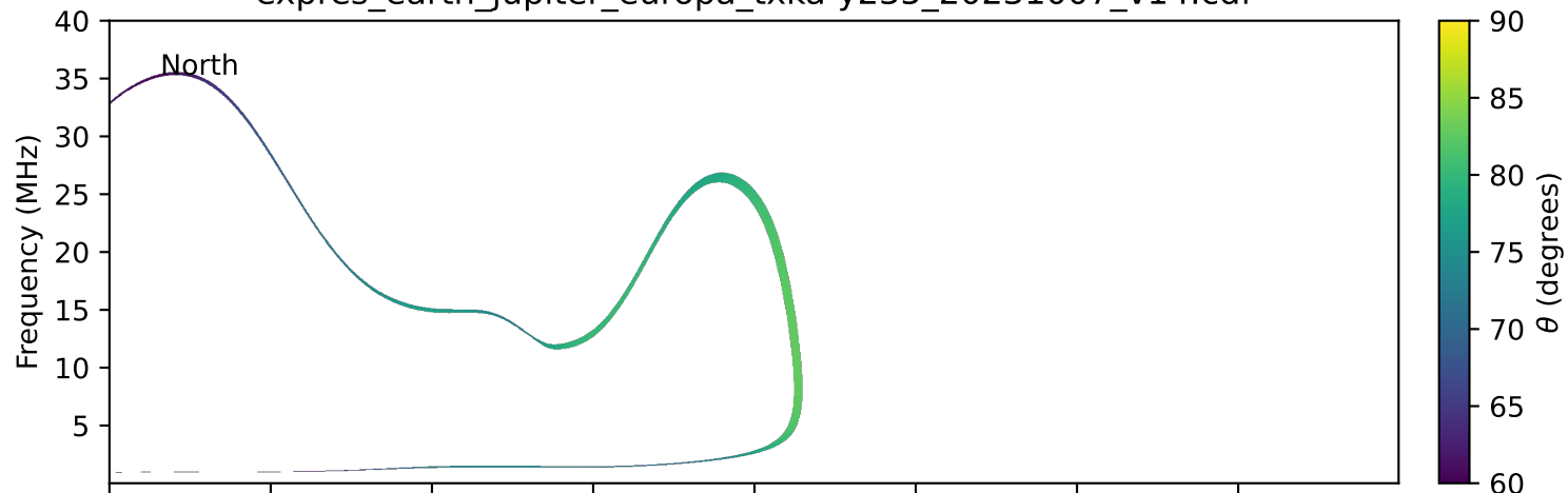
expres_earth_jupiter_europa_txka-y235_20231007_v14.cdf
