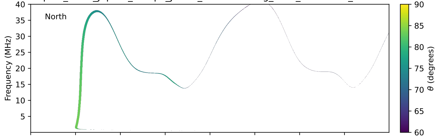
expres_earth_jupiter_europa_jrm33_lossc-wid1deg_3kev_20231020_v11.cdf
