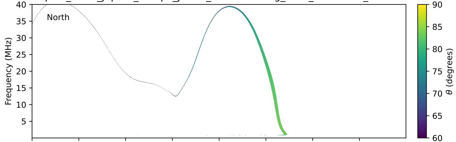
expres_earth_jupiter_europa_jrm09_lossc-wid1deg_3kev_20231021_v11.cdf
