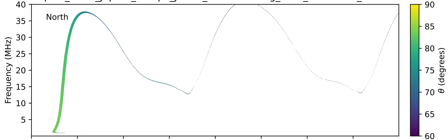
expres_earth_jupiter_europa_jrm09_lossc-wid1deg_3kev_20231013_v11.cdf
