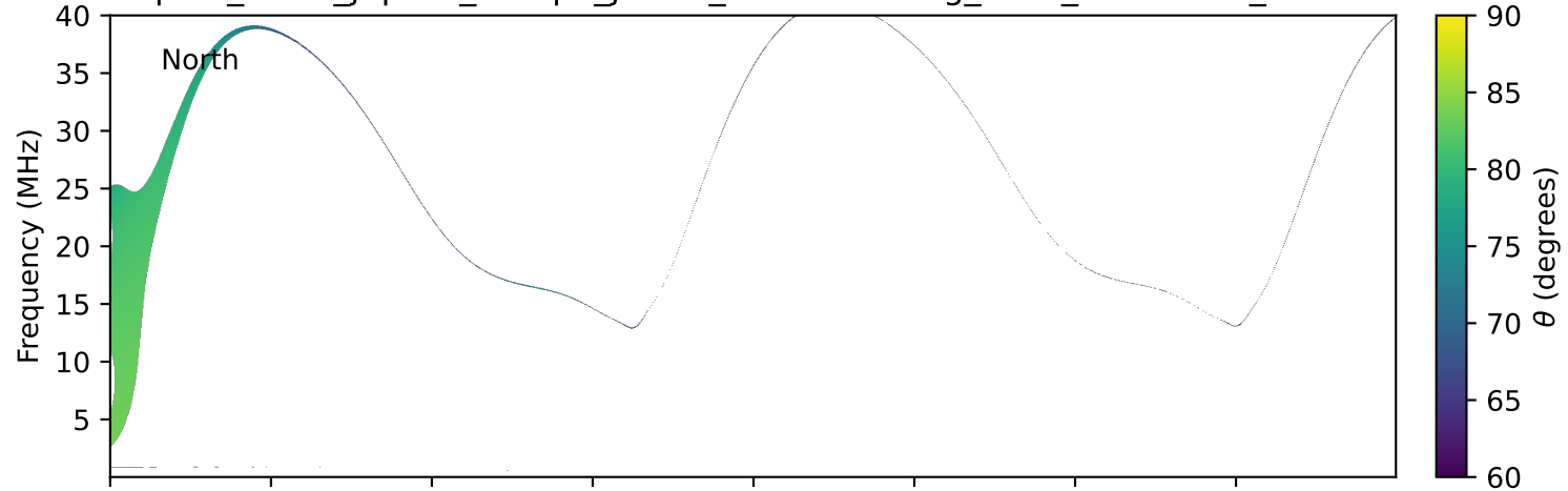
expres_earth_jupiter_europa_jrm09_lossc-wid1deg_3kev_20231006_v11.cdf
