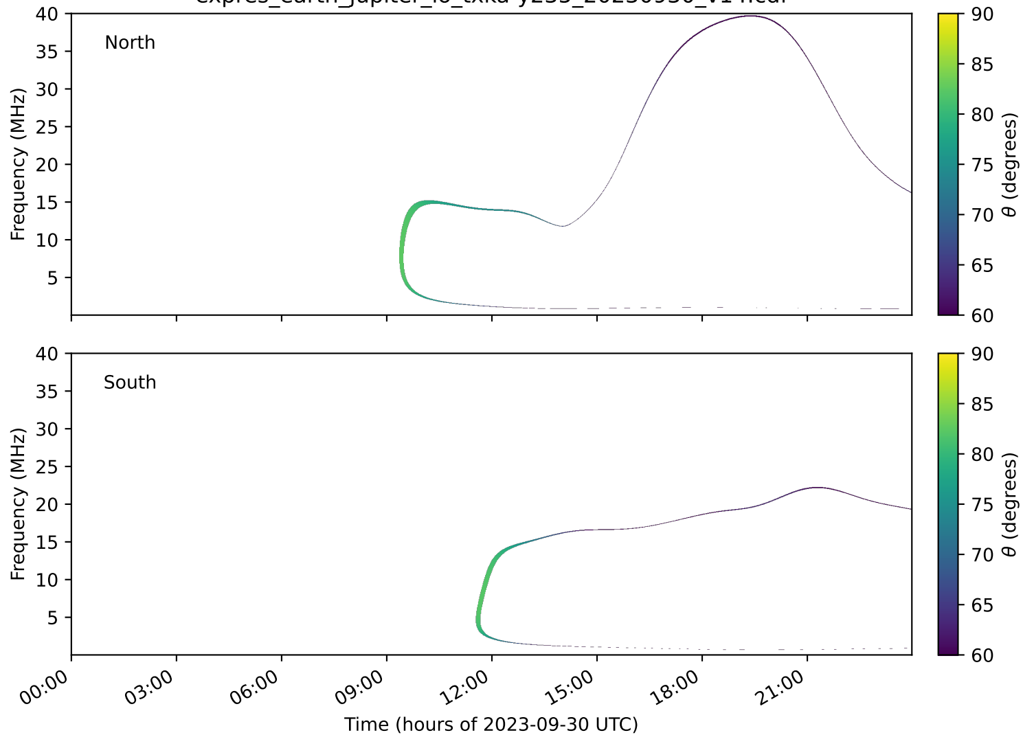
expres_earth_jupiter_io_txka-y235_20230930_v14.cdf
