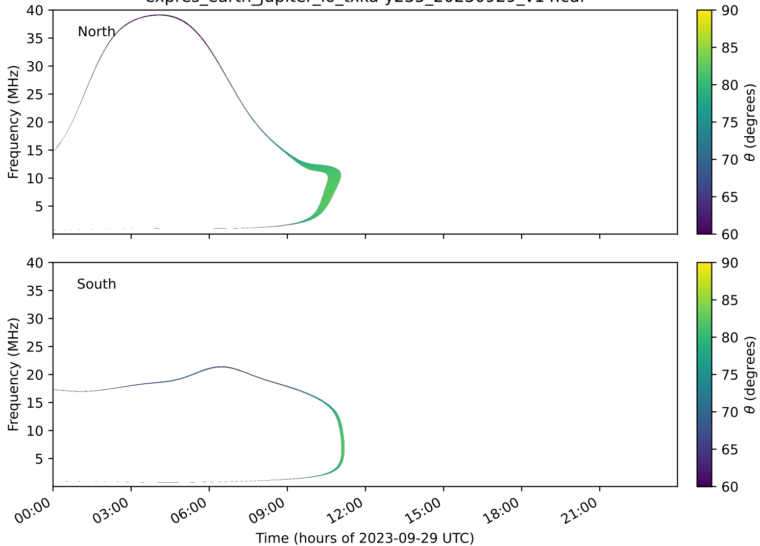
expres_earth_jupiter_io_txka-y235_20230929_v14.cdf
