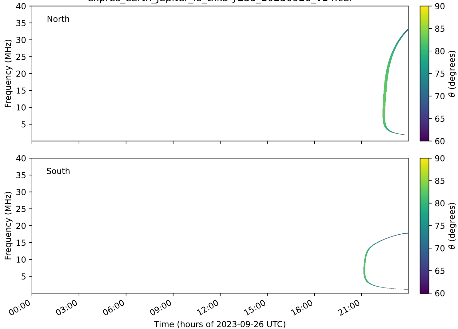
expres_earth_jupiter_io_txka-y235_20230926_v14.cdf
