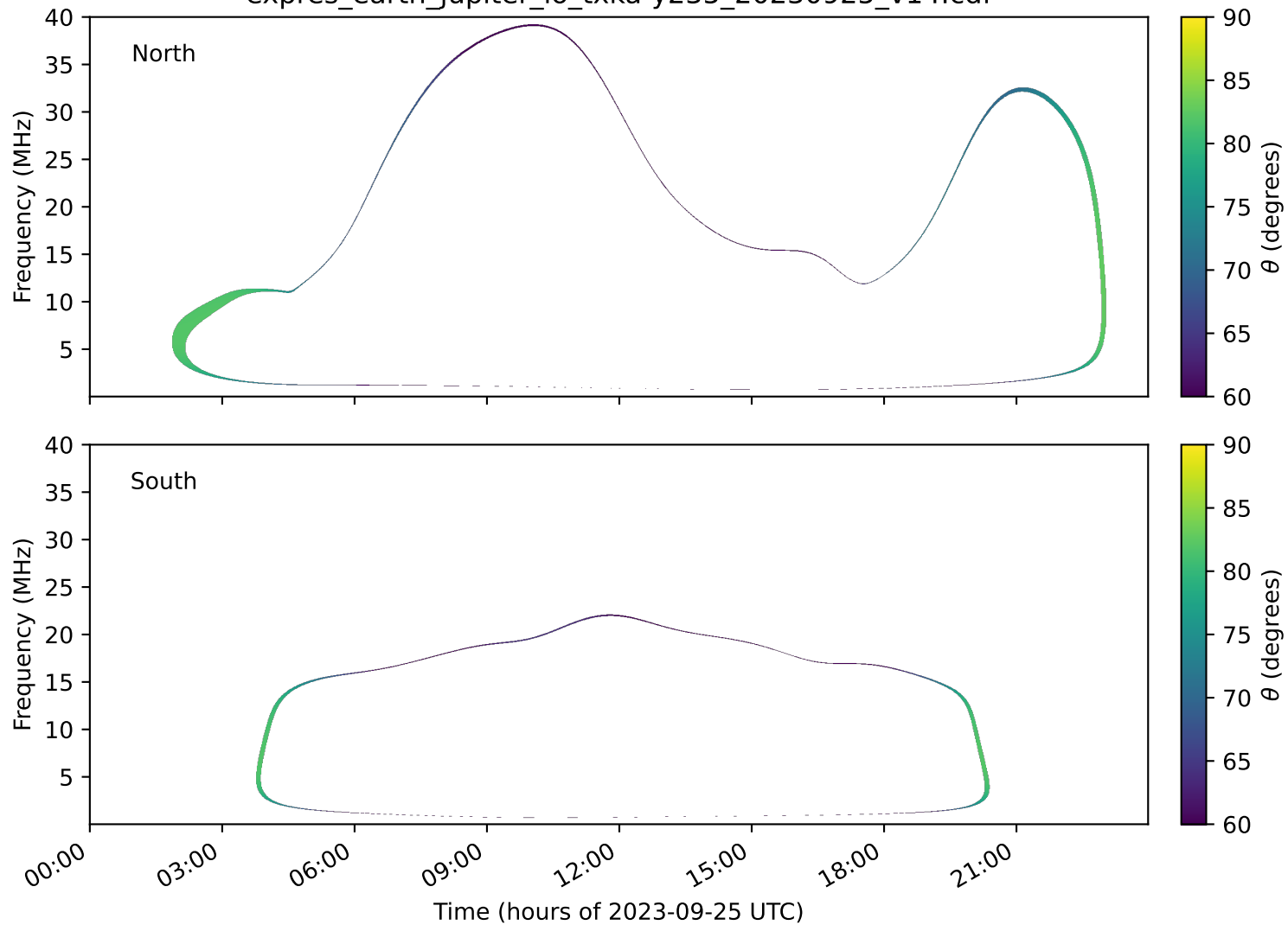
expres_earth_jupiter_io_txka-y235_20230925_v14.cdf
